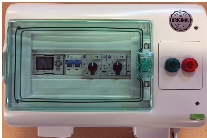
Biovac pumpestyringspanel
